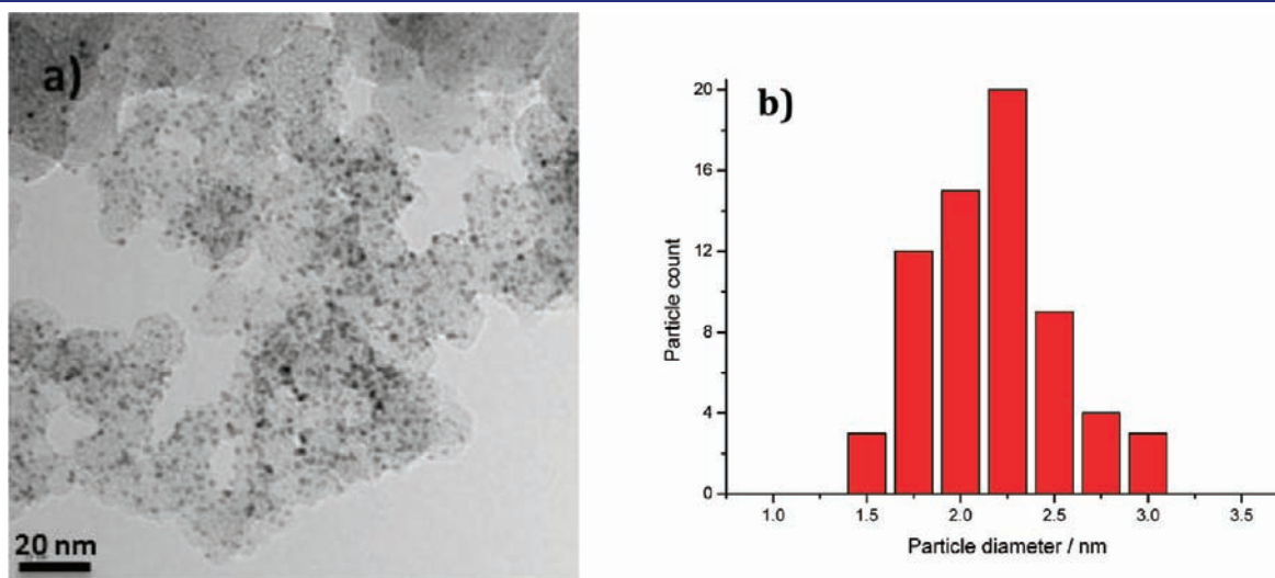
Figure 2. (a) TEM micrographs of the 4 wt % Au/C catalyst powder and (b) the particle size distribution determined by analysis of the TEM image.
