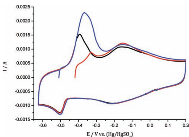
Figure 11. Stripping voltammograms for the 4 wt % Au/C electrode in 0.5 M H 2 SO 4 and 2 mM CuSO 4 at a sweep rate of 5 mV s -1 . Standard voltammogram (black), stripping after -0.42 V hold for 30 min (red), and stripping after -0.51 V hold for 30 min (blue).
